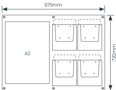
Acrylic Back Panel
